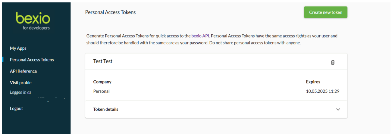
Fig 27 – Token generation
